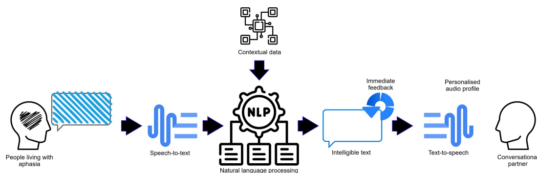
Figure 2. Overview of the Revolutionizing Speech Enhancement in Aphasia Using Knowledgeable-AI (R-SPEAK) system workflow for enhancing communication in people with aphasia. NLP: natural language processing.
