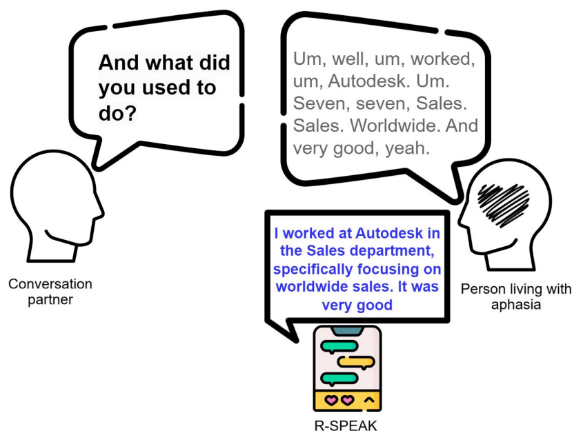
Figure 1. Example of how Revolutionizing Speech Enhancement in Aphasia Using Knowledgeable-AI (R-SPEAK) converts real-world aphasic speech into comprehensible speech.
