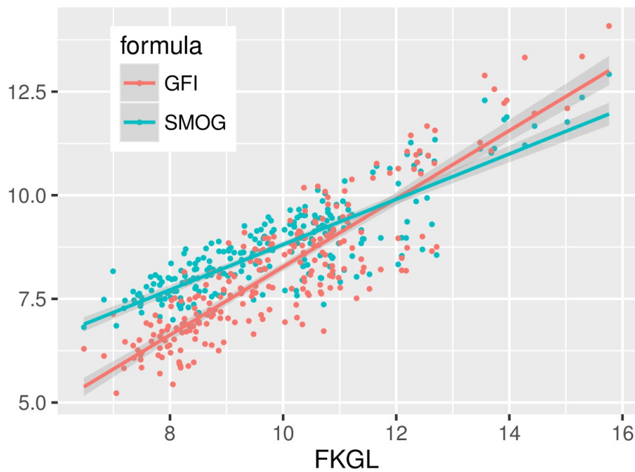
Figure A3-2: Scatter plot of SMOG and GFI scores against FKGL on med genre text.
