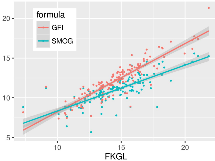
Figure A3-1: Scatter plot of SMOG and GFI scores against FKGL on wiki genre text.
